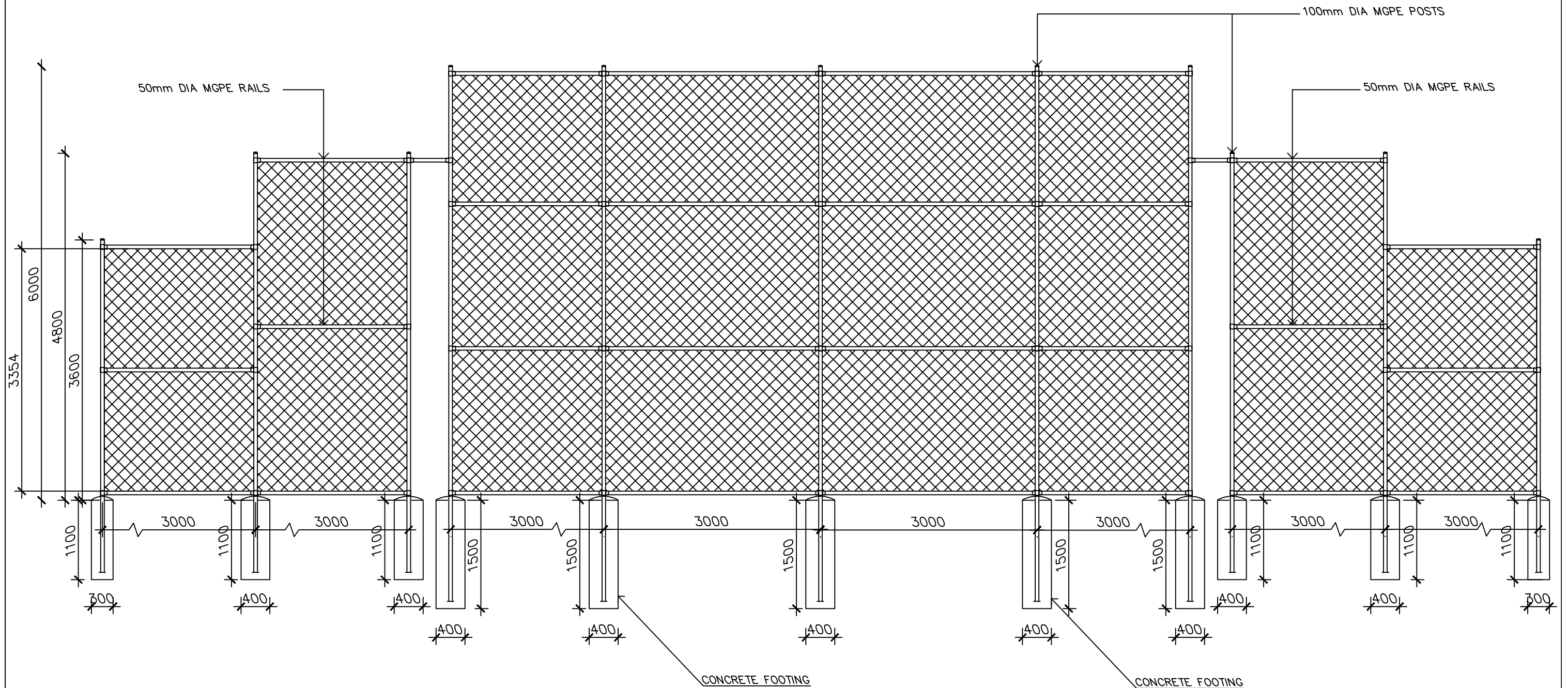
1 ELEVATION — NTS
